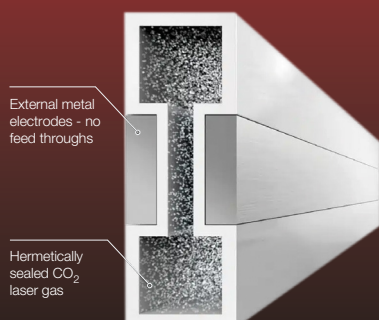
Ceramic CO 2 Laser
